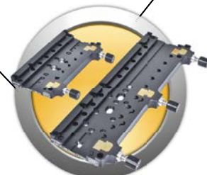
Baader Pan EQ dual clamps to hold 44mm EQ-dovetails, bottom has 3" dovetail built-in with brass clamping blocks 230 / 370 mm long #2451566 / #2451565
